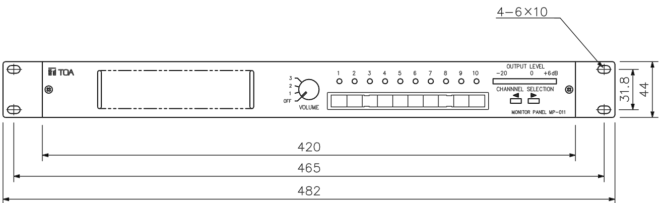
Front View
