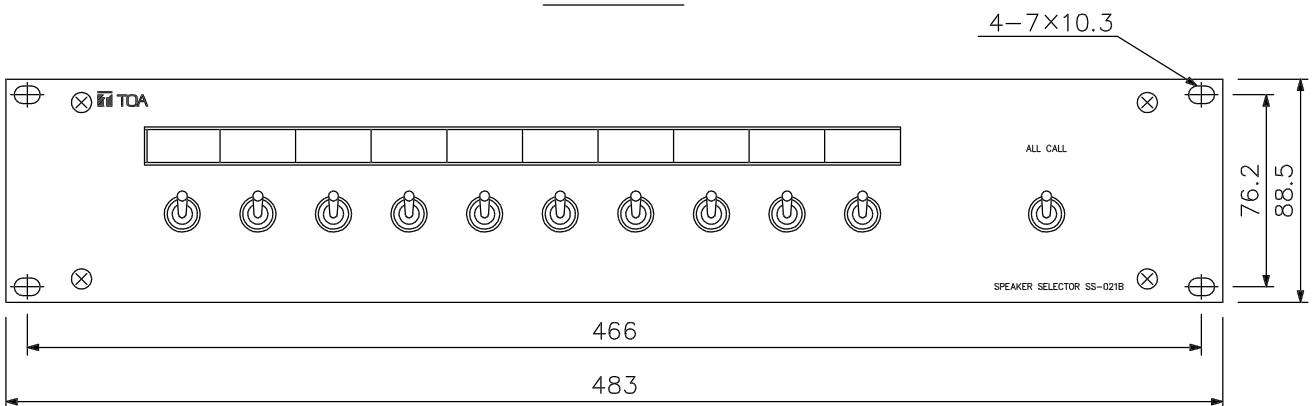
Front View
