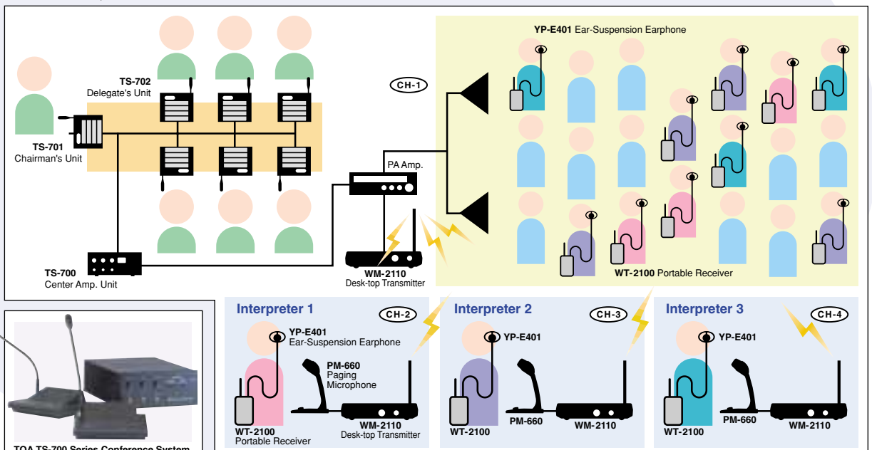
TOA TS-700 Series Conference System
