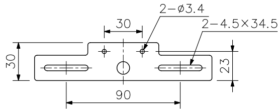
Magnified view of preinstalled tie-plate (SCALE:1/3)
