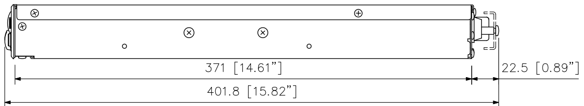
Side View
