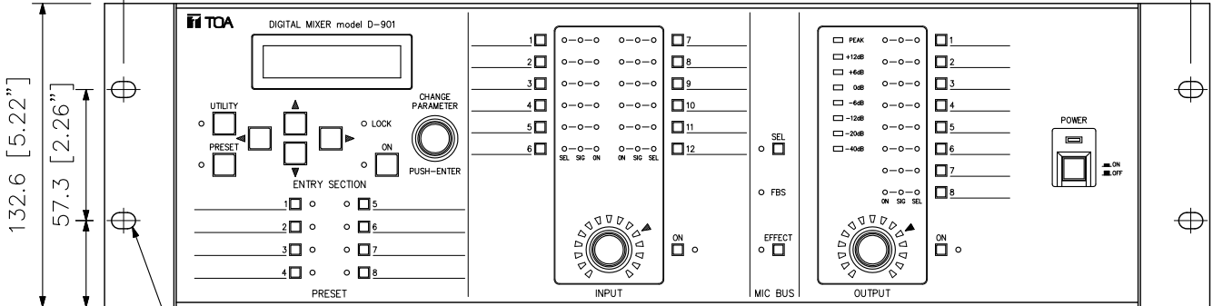
Front View
