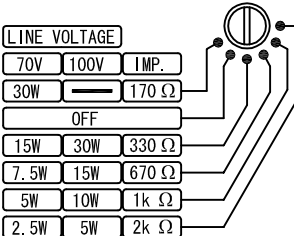
Impedance Selection
